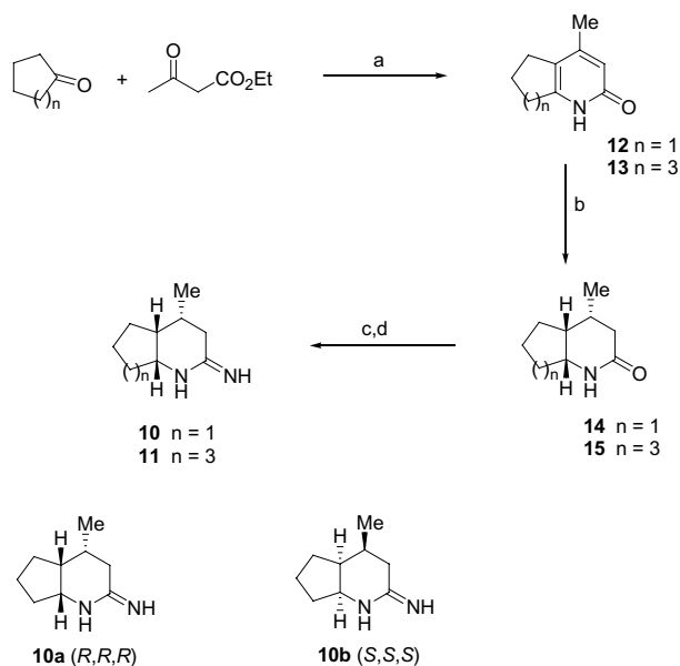
Scheme 3. (a) \text{NH}_4\text{OAc} , EtOH, 80 °C; (b) \text{H}_2 , \text{PtO}_2 , HOAc; (c) \text{Me}_3\text{OBF}_4 , \text{CH}_2\text{Cl}_2 , rt; (d) \text{NH}_4\text{Cl} , EtOH, 80 °C.
