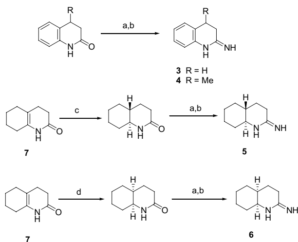
Scheme 1. Reagents and conditions: (a) Me 3 OBf 4 , CH 2 Cl 2 , rt; (b) NH 4 Cl, EtOH, 80 °C; (c) HCOONa, HCOOH, 100 °C; (d) H 2 , Pd/C, dioxane, ethanol.
