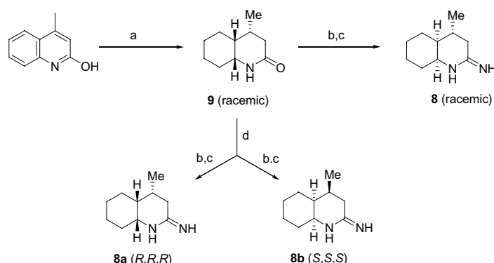
Scheme 2. Reagents and conditions: (a) H 2 , PtO 2 , HOAc; (b) Me 3 OBf 4 , CH 2 Cl 2 , rt; (c) NH 4 Cl, EtOH, 80 °C; (d) resolution on Chiralcel OD column, 10% isopropanol/hexane.
